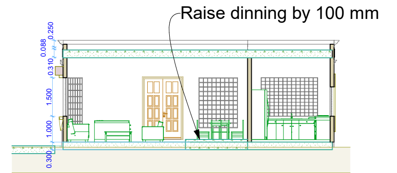
SECTION-02
