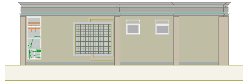
NORTH ELEVATION
